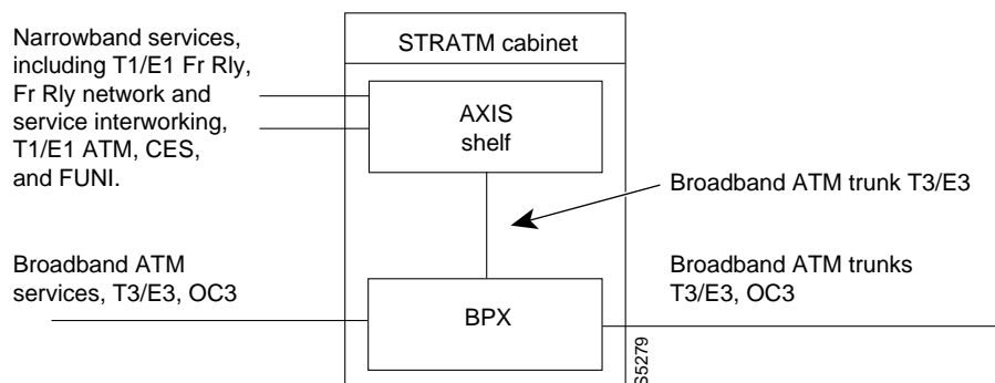
Figure 15-1 Tiered Network
