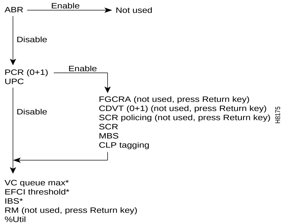
Figure 10-2 Prompt Sequence for a VBR/ATFR Connection
