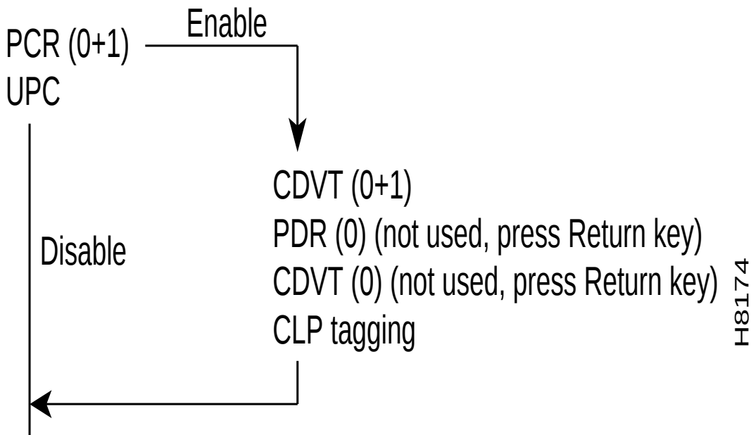
Figure 10-1 Prompt Sequence for a CBR Connection
