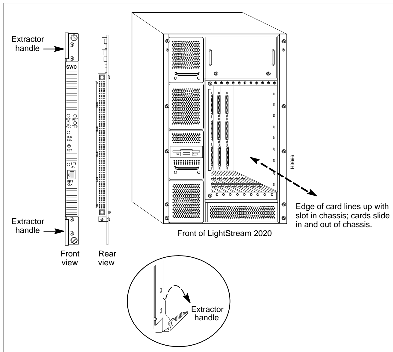
Figure 5-1 LS2020 Switch Card Replacement
