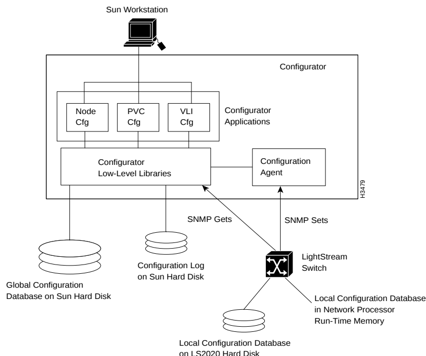
Figure 1-1 Configurator Block Diagram
