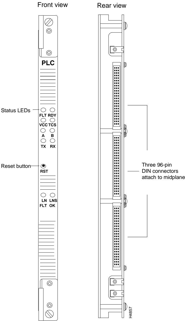
Figure 2-6 Packet Line Card
