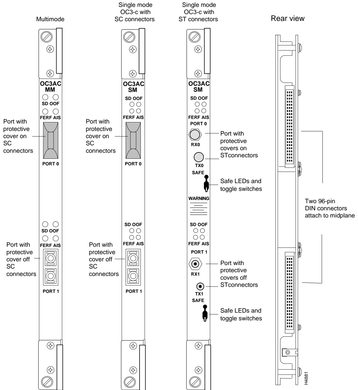
Figure 2-3 OC-3c Multimode and Single Mode Access Cards
