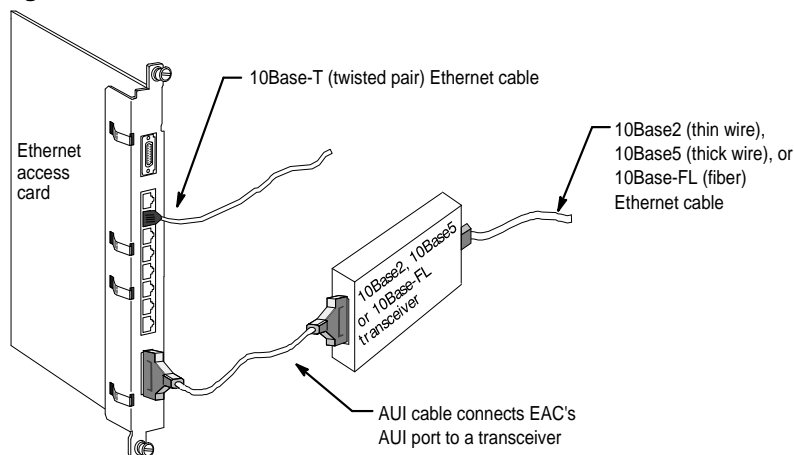
Figure 2-7 10Base-T, 10Base5, 10Base2, and 10Base-FL Connections
