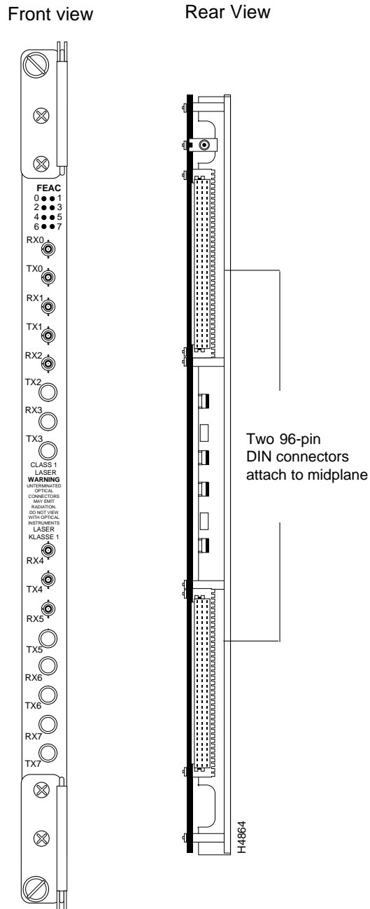
Figure 2-9 Fiber Ethernet Access Card
