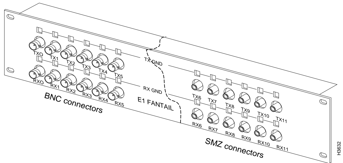
Figure 2-15 E1 Fantails Showing BNC and SMZ Connectors
