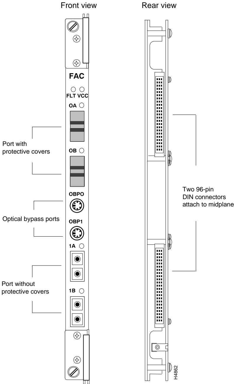
Figure 2-11 FDDI Access Card
