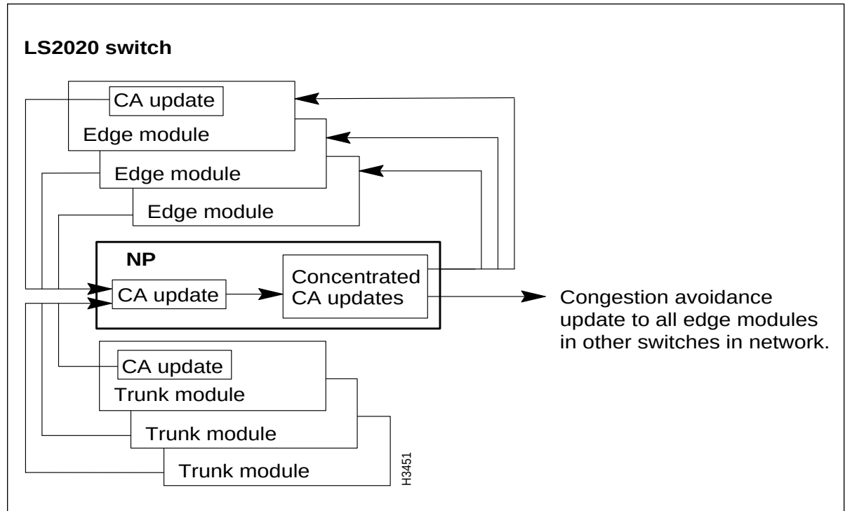
Figure 4-4 Rate-Based Congestion Avoidance Feedback Loop
