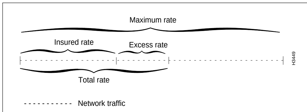
Figure 4-2 Relationship among VCC Traffic Policing Parameters
