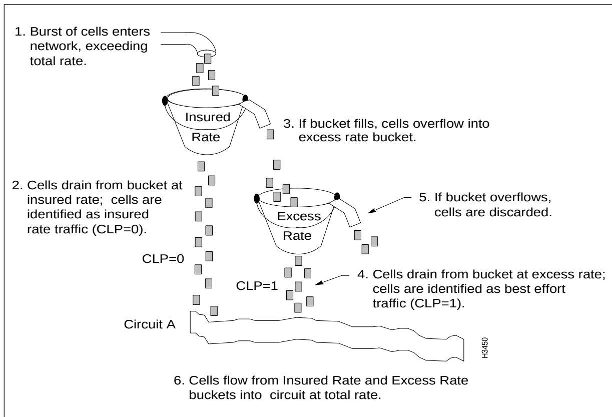
Figure 4-3 Dual Leaky Bucket Traffic Policer
