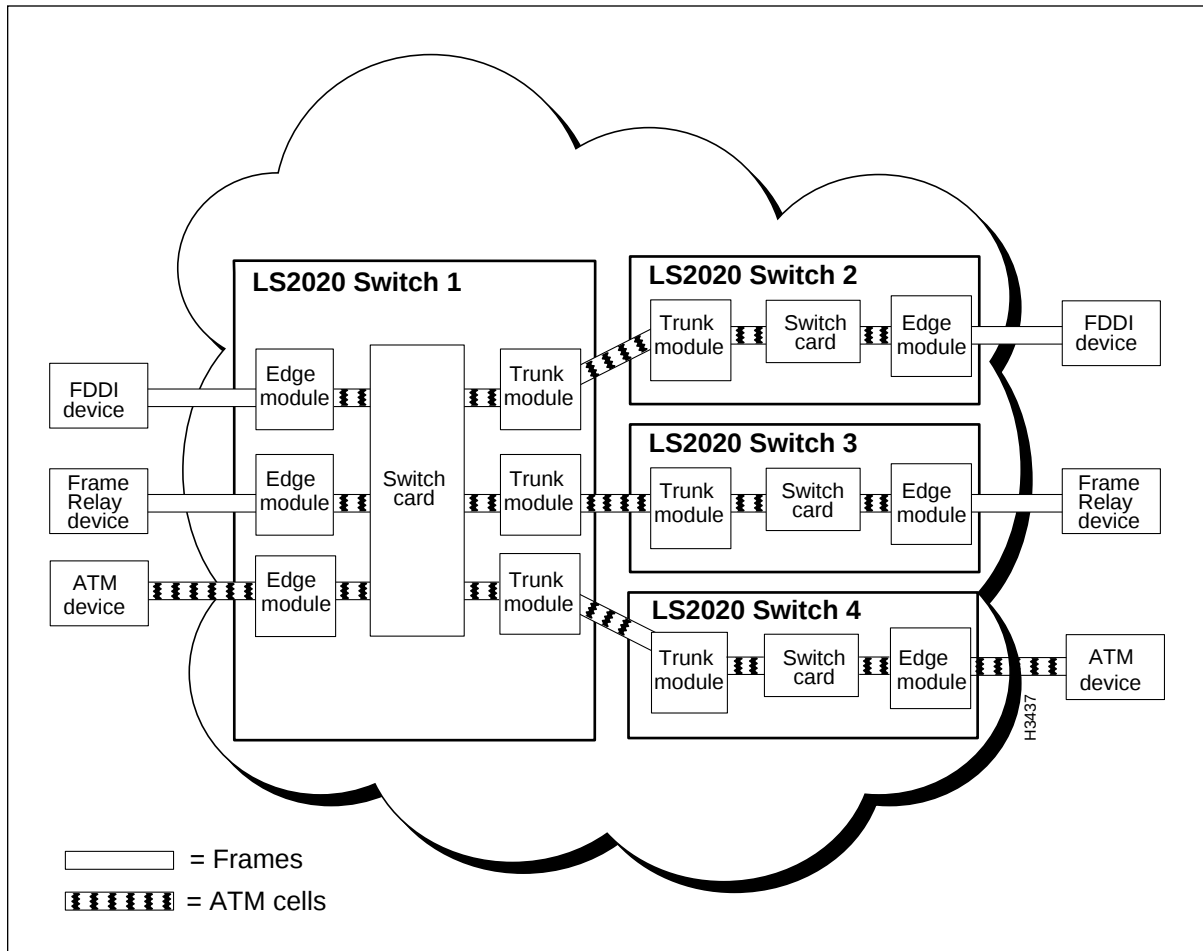
Figure 2-3 Simplified View of LS2020 Network
