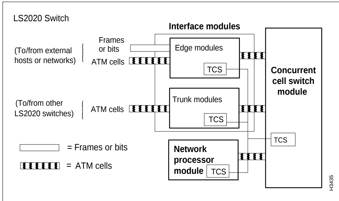
Figure 2-1 Key Components of LS2020 Switch
