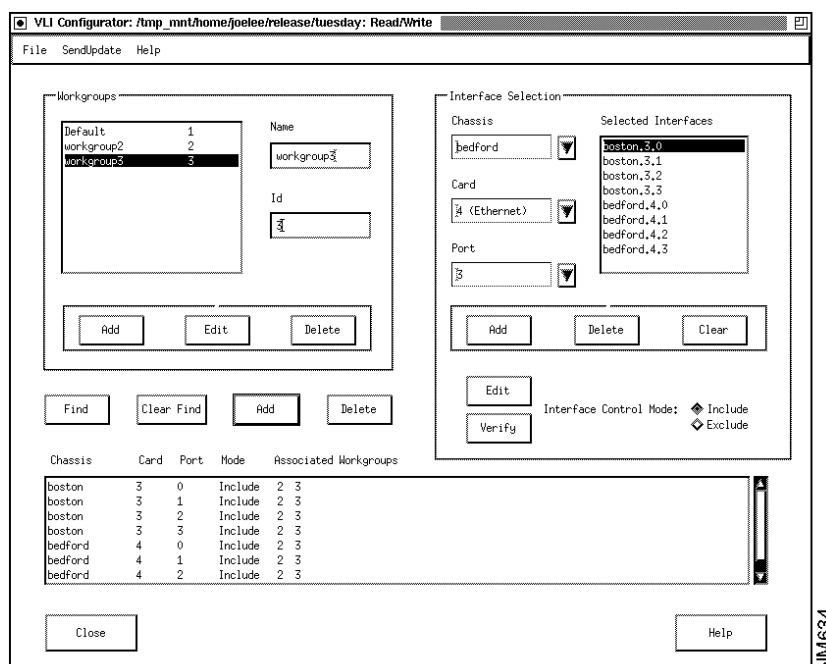
Figure 3-37 VLI Configuration Dialog Box with Two Defined Workgroups
