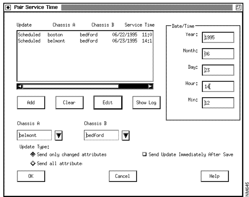
Figure 3-39 Sample Update Time Dialog Box for PVC Configurator
