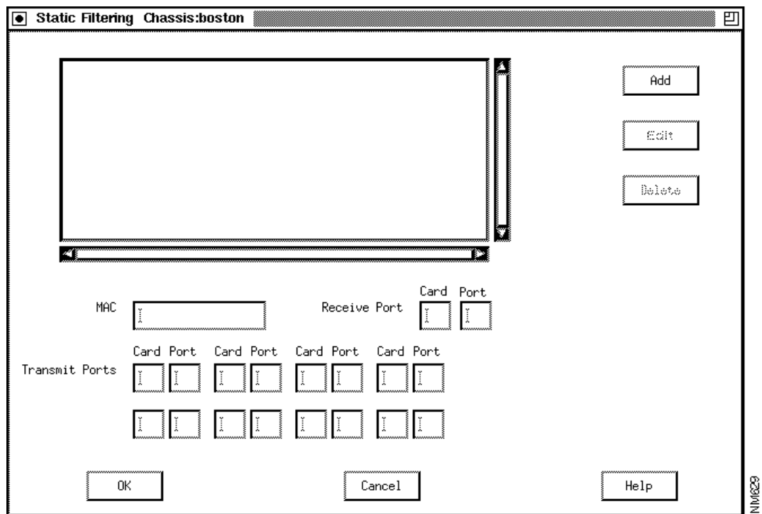
Figure 3-31 Static Filtering Dialog Box
