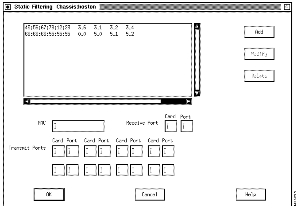
Figure 3-32 Static Filtering Dialog Box with Two Multicast Filters Defined
