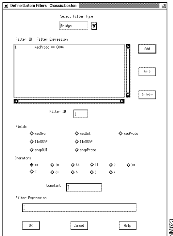
Figure 3-26 Sample Custom Filter Definition
