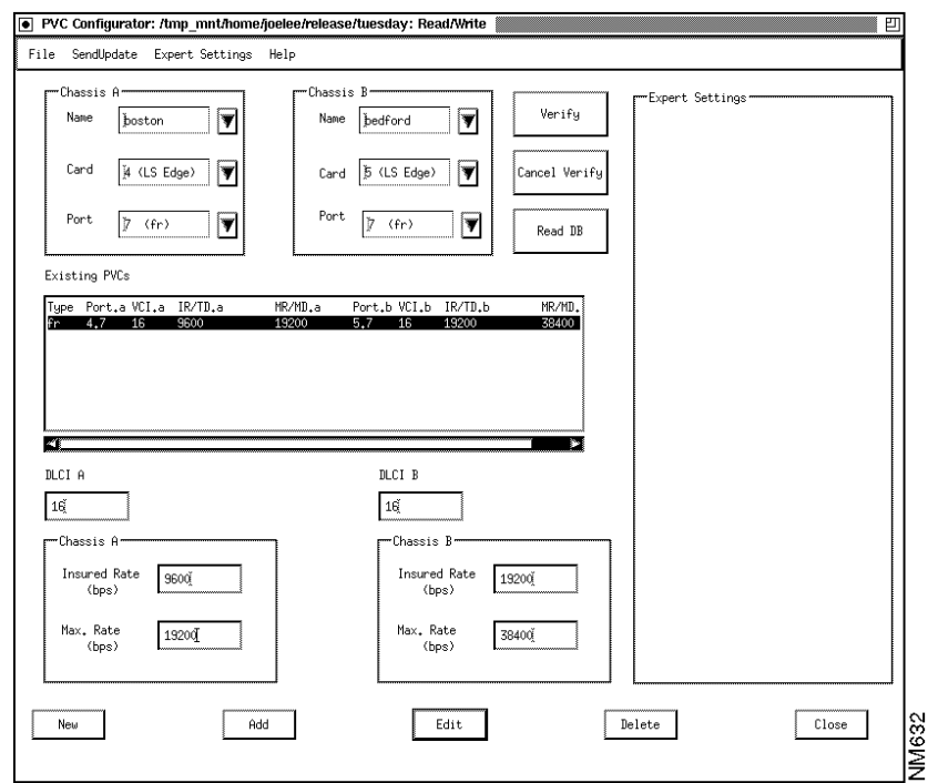
Figure 3-34 PVC Dialog Box with One Frame Relay Circuit Defined
