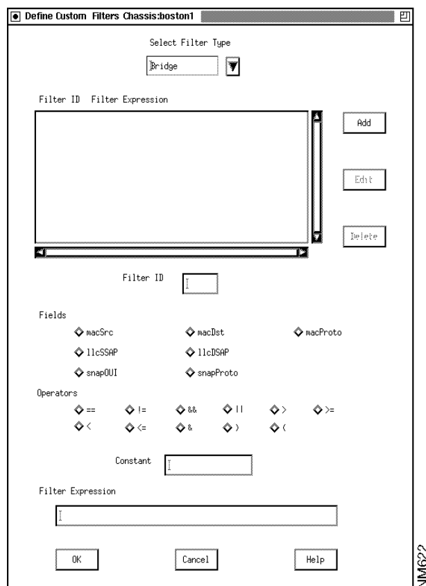
Figure 3-25 Define Custom Filters Dialog Box
