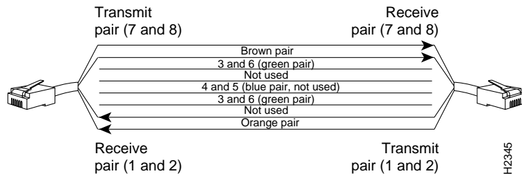
Figure E-2 Straight-Through Cable Pinout
