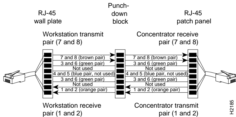
Figure F-3 Punch-Down Block Connections
