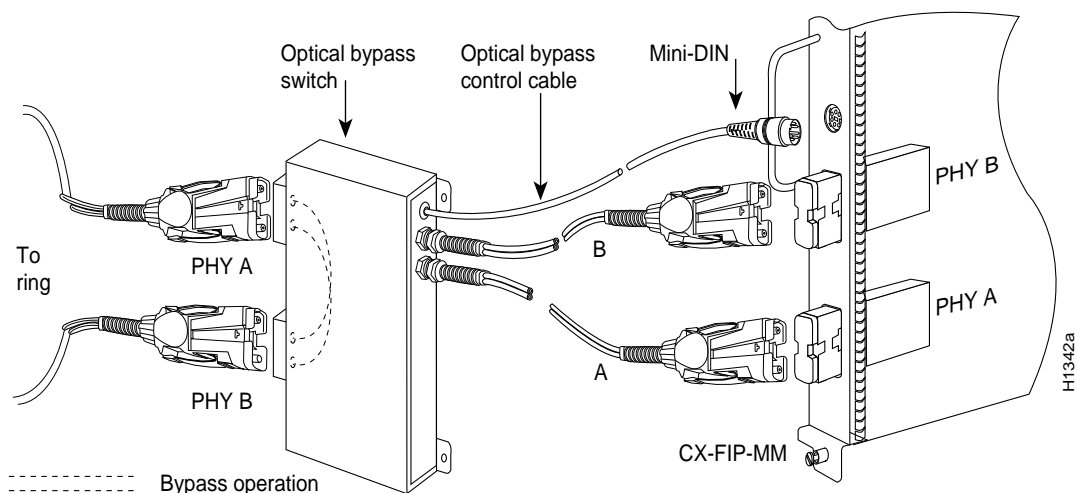
Figure 3-15 FDDI Connection with Optical Bypass (CX-FIP-MM)
