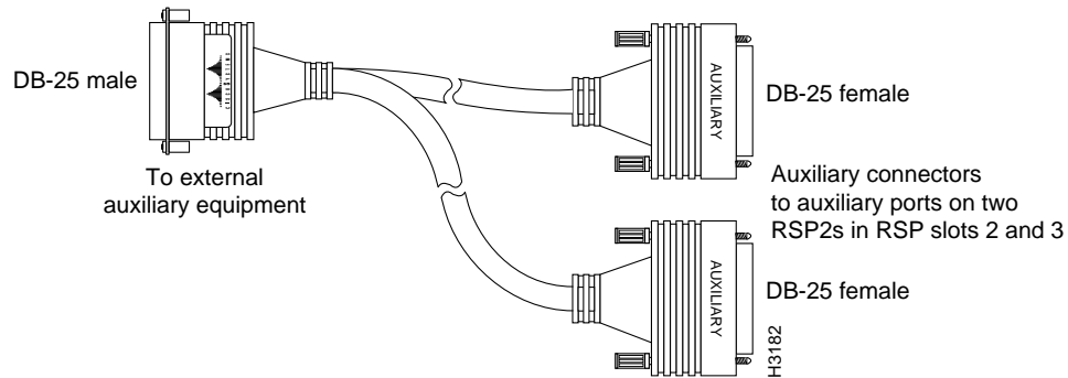
Figure 3-23 Auxiliary Y Cable
