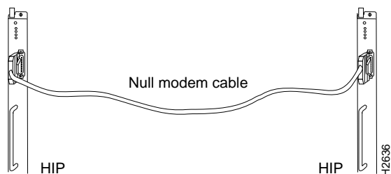
Figure 3-19 HSSI Null Modem Connection (Two HIPs Connected Back to Back)
