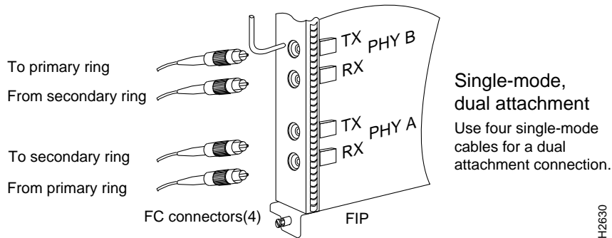
Figure 3-12 Dual Attachment Station (Single-Mode Fiber Network Connections)
