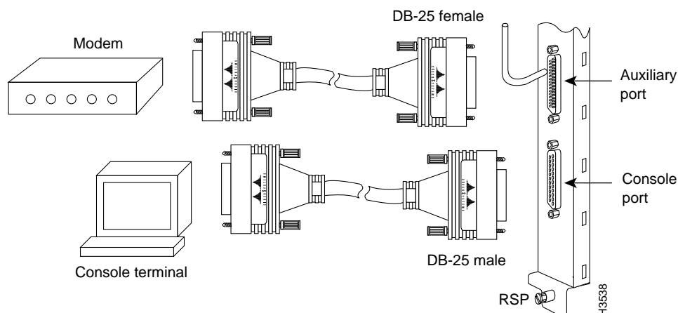
Figure 3-21 Console and Auxiliary Port Connections
