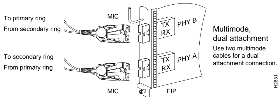
Figure 3-13 Dual Attachment Station (Multimode Fiber Network Connections)
