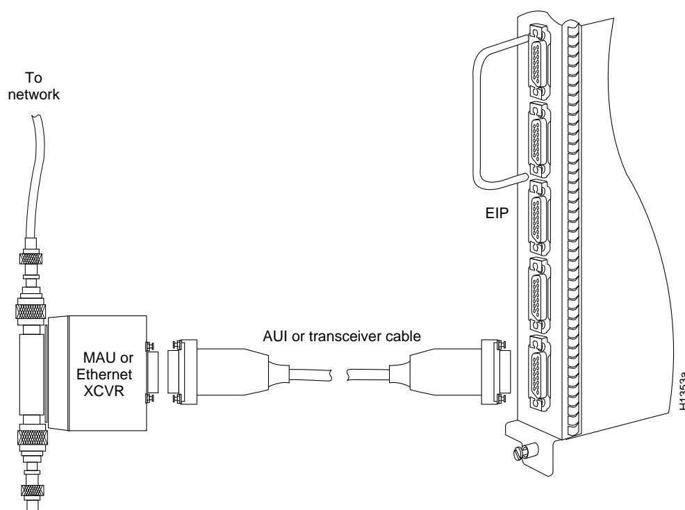
Figure 3-6 Ethernet Connections
