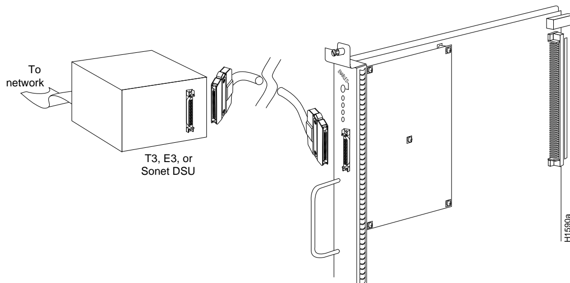
Figure 3-18 HSSI Network Connection
