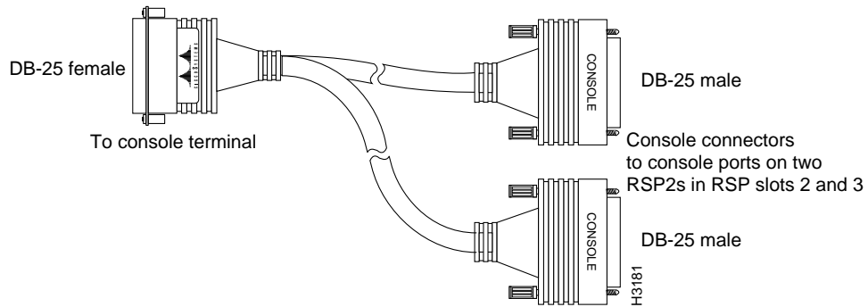
Figure 3-22 Console Y Cable
