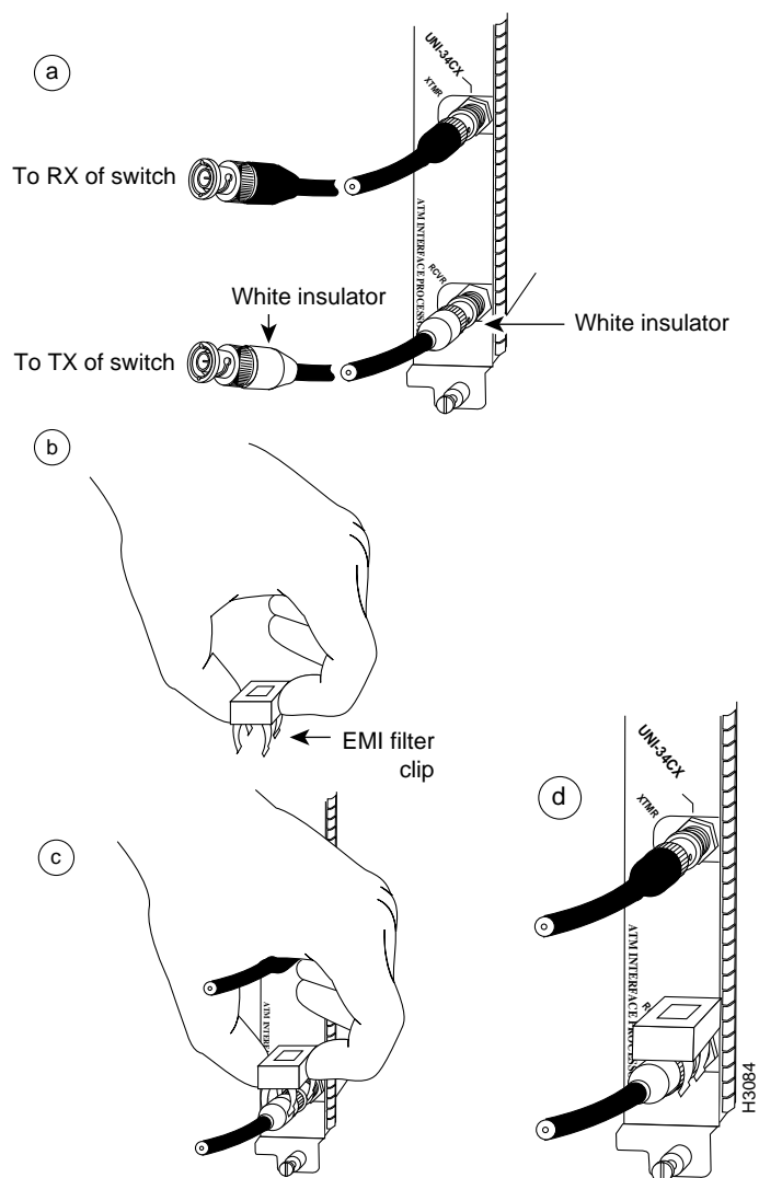
Figure 3-5 Installing the CAB-ATM-DS3/E3 Cable and EMI Filter Clip Assembly
