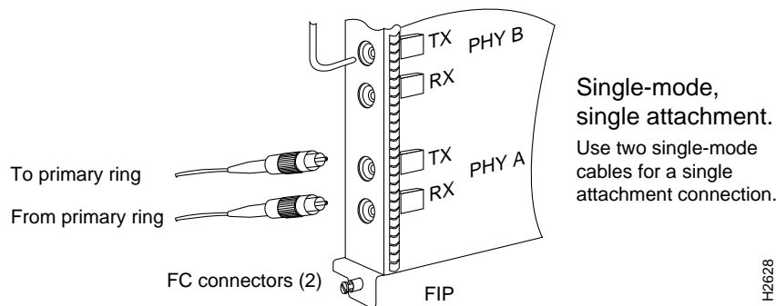
Figure 3-9 Single Attachment Station (Single-Mode Fiber Network Connections)
