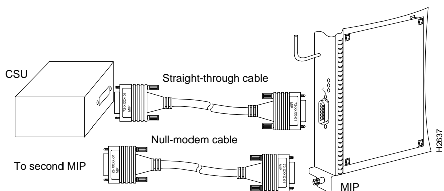
Figure 3-20 MIP Connections
