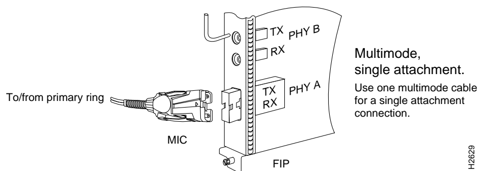
Figure 3-10 Single Attachment Station (Multimode Fiber Network Connections)
