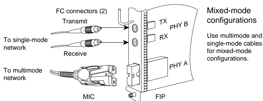
Figure 3-14 FDDI Dual Attachment Network Connections (Single-Mode and Multimode)
