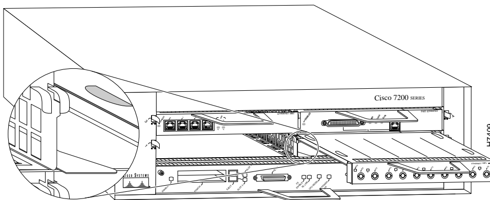
Figure 6-3 Aligning the Port Adapter Metal Carrier Between the Slot Guides
