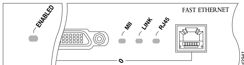
Figure B-7 FEIP LEDs
