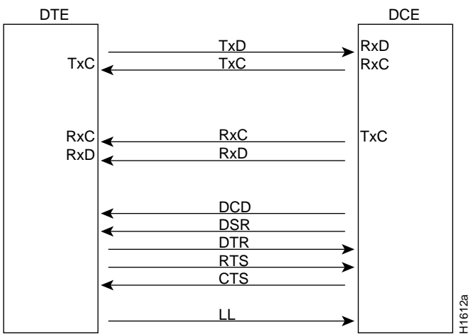
Figure B-11 DTE to DCE Signals
