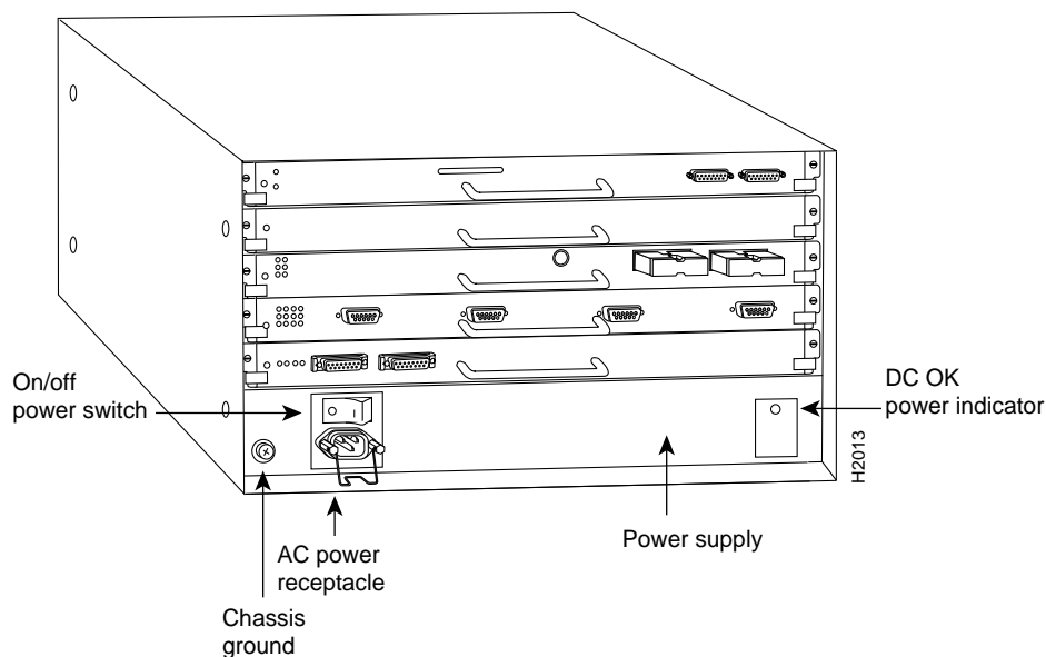
Figure B-1 DC OK LED—AC-Input Power Supply Shown
