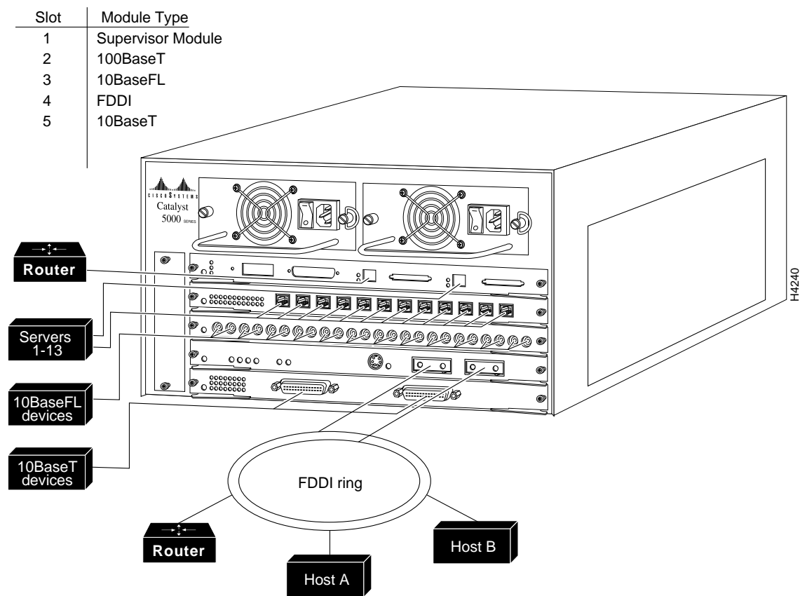
Figure 6-35 Single Catalyst 5000 Series Switch Configuration
