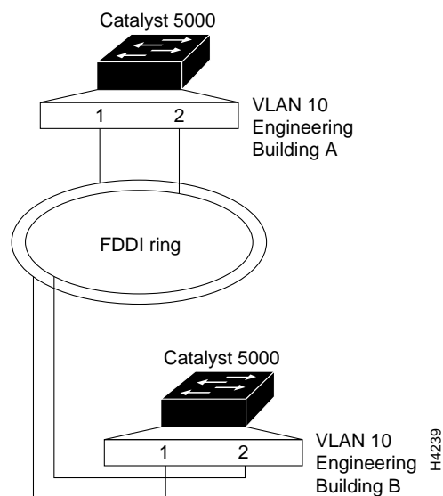
Figure 6-36 Multiple Catalyst 5000 VLAN Configuration without Trunking
