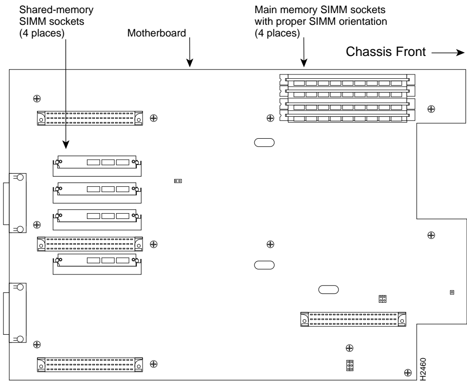
Figure 8 Original Cisco 4000 SIMM Locations
