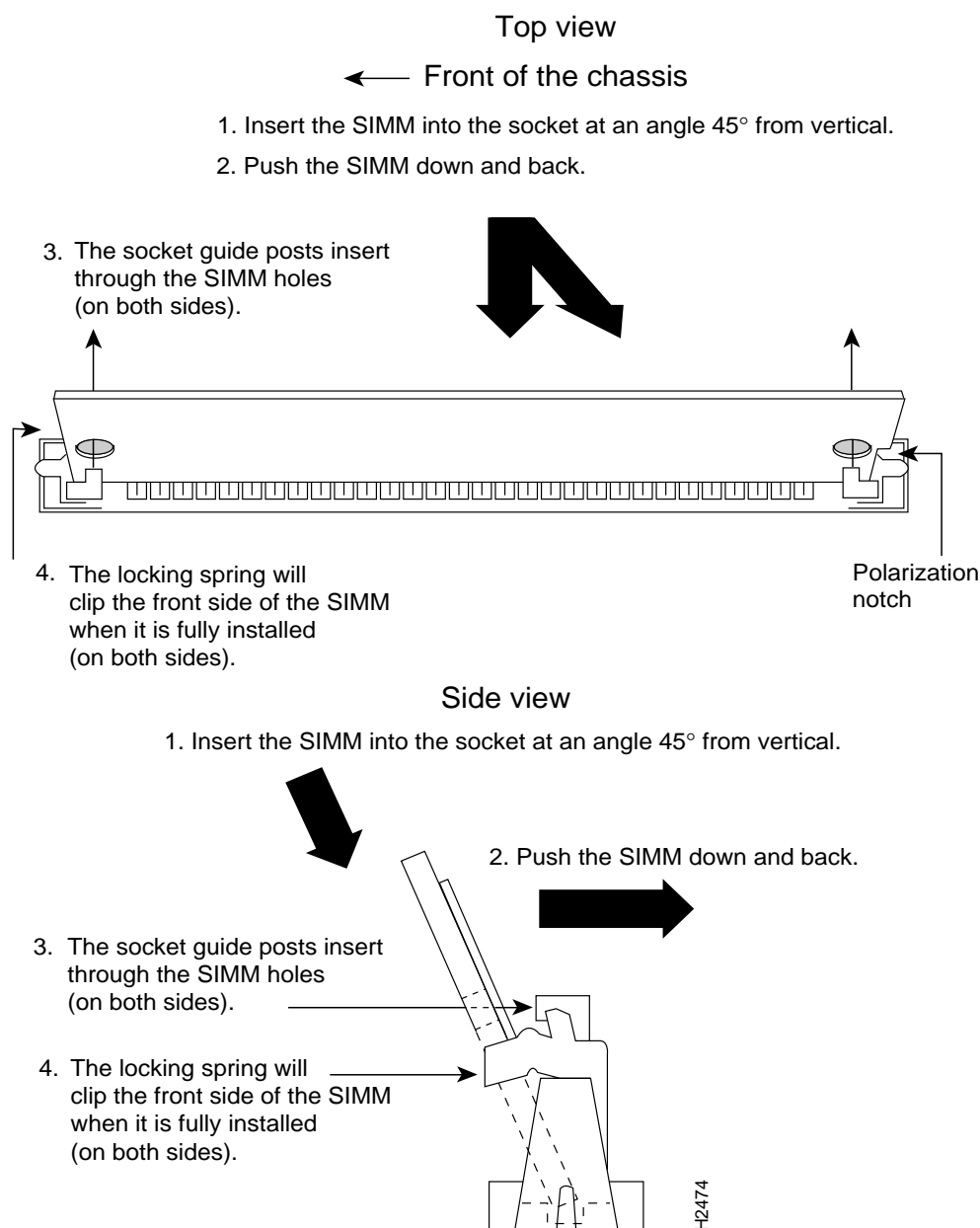
Figure 15 Inserting Flash Memory SIMMs in the Cisco 4000-M
