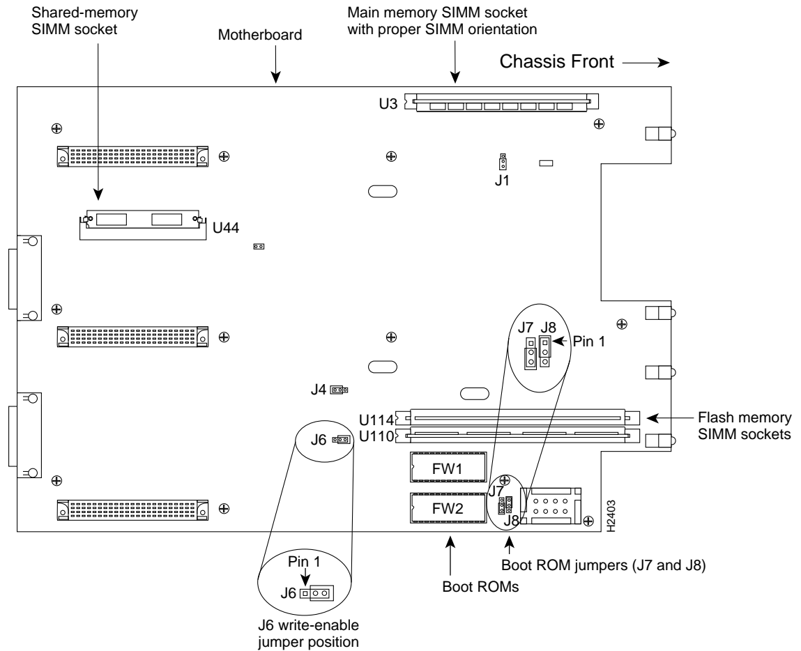
Figure 10 Cisco 4000-M SIMM Locations
