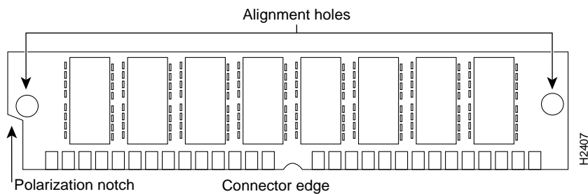
Figure 11 Cisco 4000-M Main Memory SIMM
