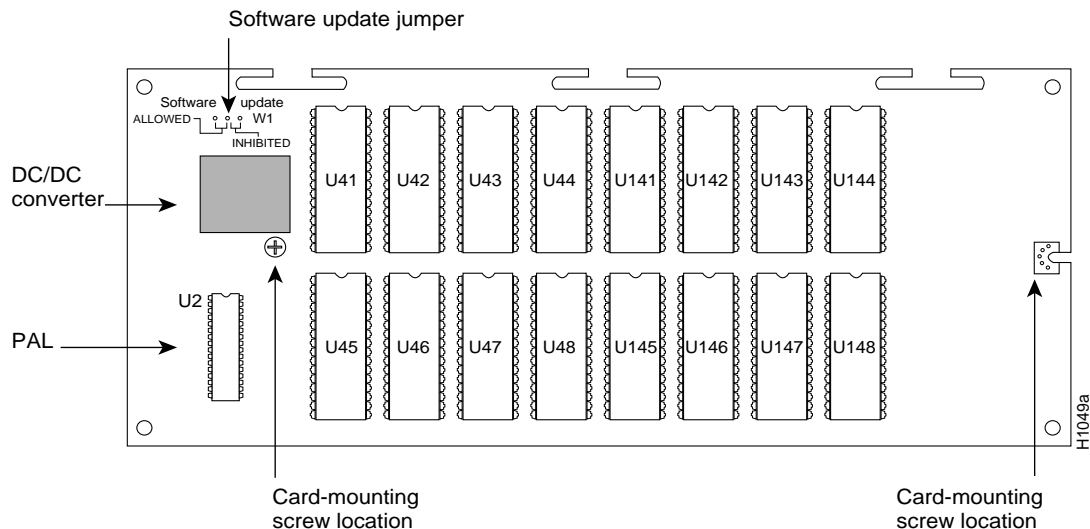
Figure 6 Flash EPROM Card
