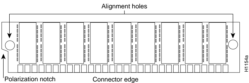
Figure 9 Original Cisco 4000 Main Memory SIMM
