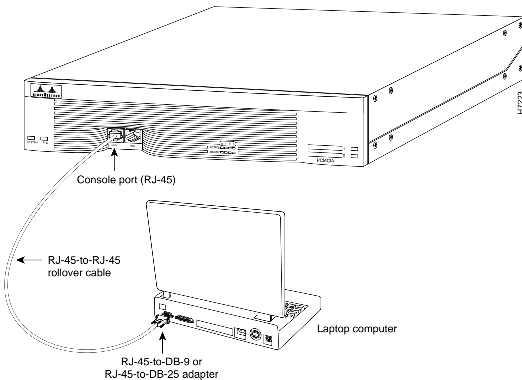
Figure E-1 Connecting the Console
