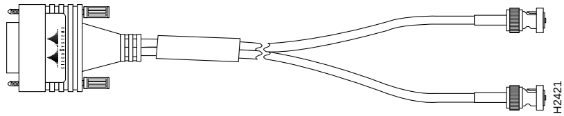
Figure C-13 E1 Interface Cable for 75-Ohm, Unbalanced Connections with BNC Connectors
