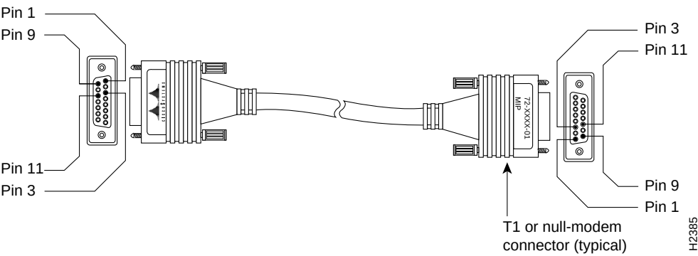
Figure C-9 T1 Interface Cable
