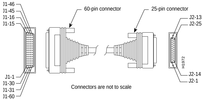
Figure C-6 EIA-530 Serial Cable Assembly
