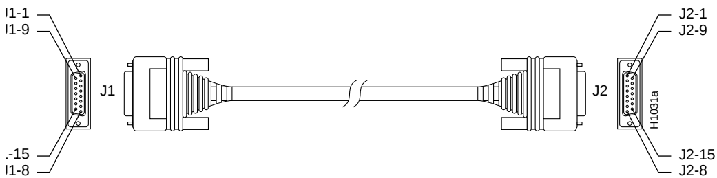
Figure C-7 Ethernet AUI Cable Assembly
