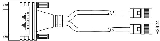
Figure C-11 E1 Interface Cable for 120-Ohm, Balanced Connections with Twinax Connectors
