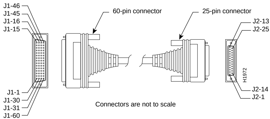
Figure C-2 EIA/TIA-232 Serial Cable Assembly
