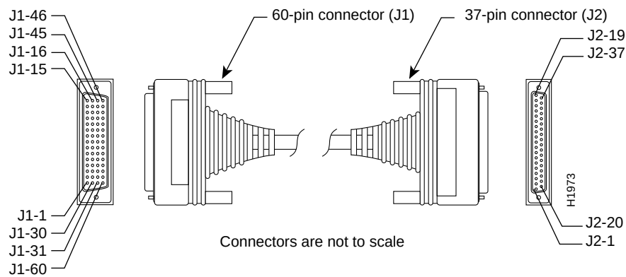
Figure C-3 EIA/TIA-449 Serial Cable Assembly
