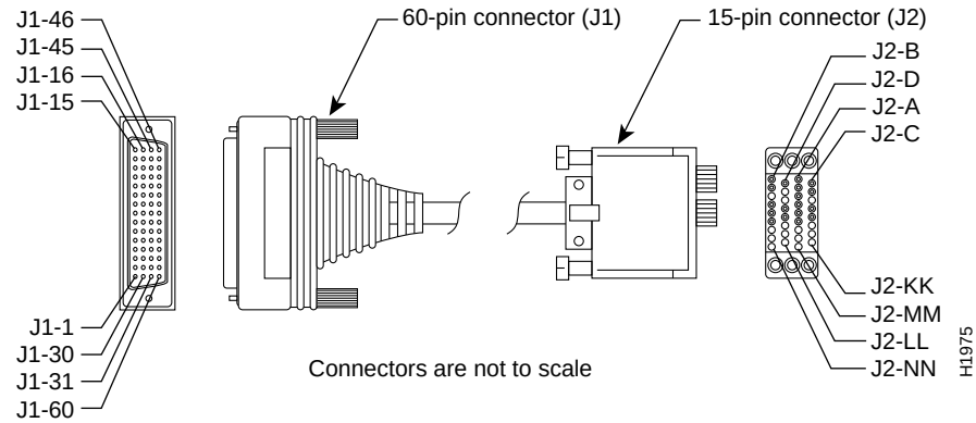
Figure C-4 V.35 Serial Cable Assembly
