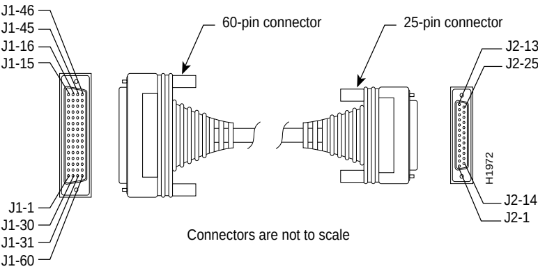
Figure D-3 EIA/TIA-232 Cable Assembly
