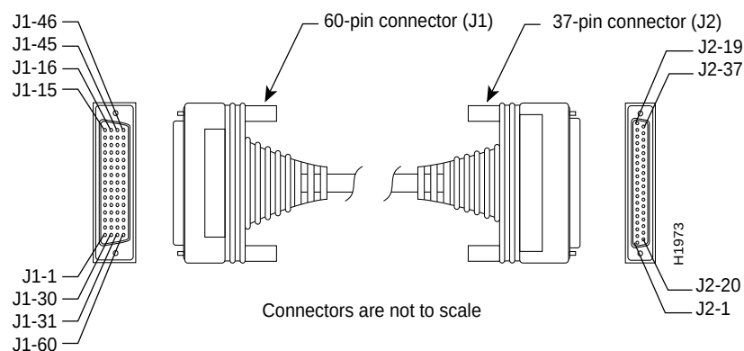
Figure D-4 EIA/TIA-449 Cable Assembly
