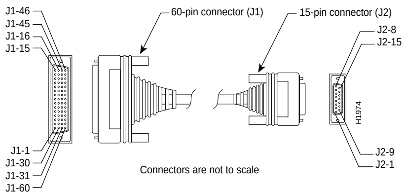
Figure D-6 X.21 Cable Assembly
