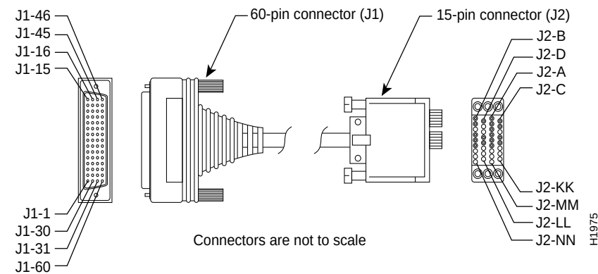
Figure D-5 V.35 Cable Assembly
