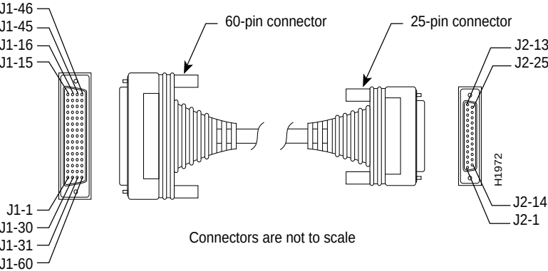
Figure D-2 EIA-530 Serial Cable Assembly
