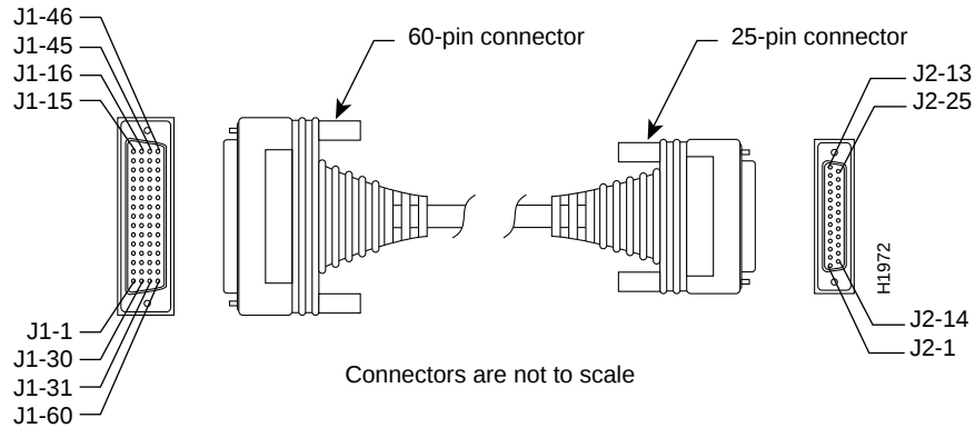
Figure C-1 EIA-530 Serial Cable Assembly
