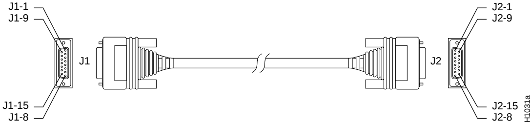
Figure C-6 Ethernet (AUI) Cable Assembly
