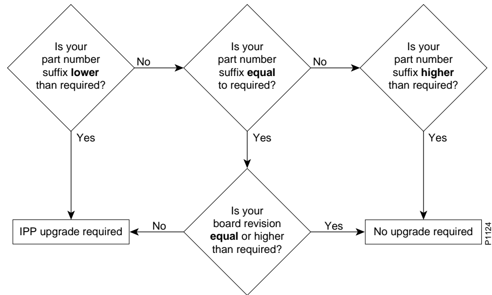
Figure 32 Determining Compatibility from Board Part Numbers and Revision Levels
