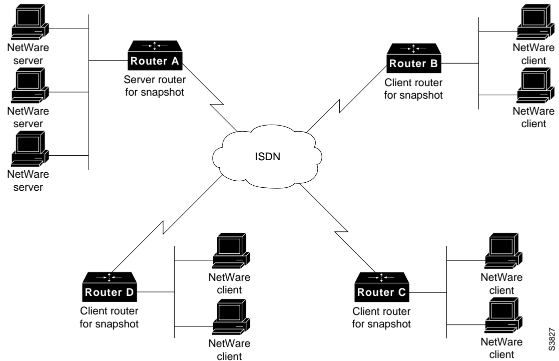
Figure 8-4 Topology of the Novell IPX Network
