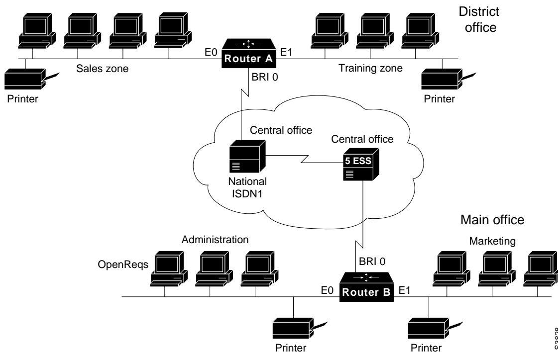
Figure 8-5 An AppleTalk Network over ISDN
