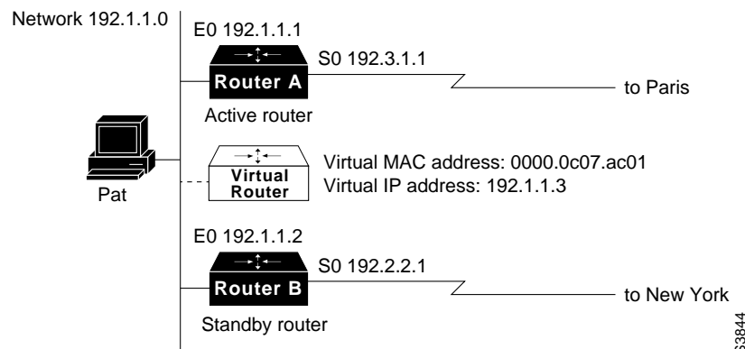
Figure 9-2 HSRP Addressing on the Tokyo Segment
