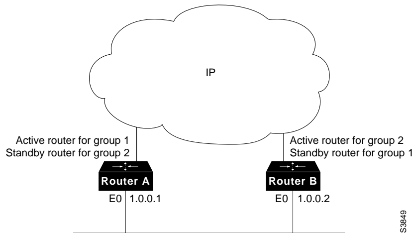
Figure 9-6 Load Sharing Example
