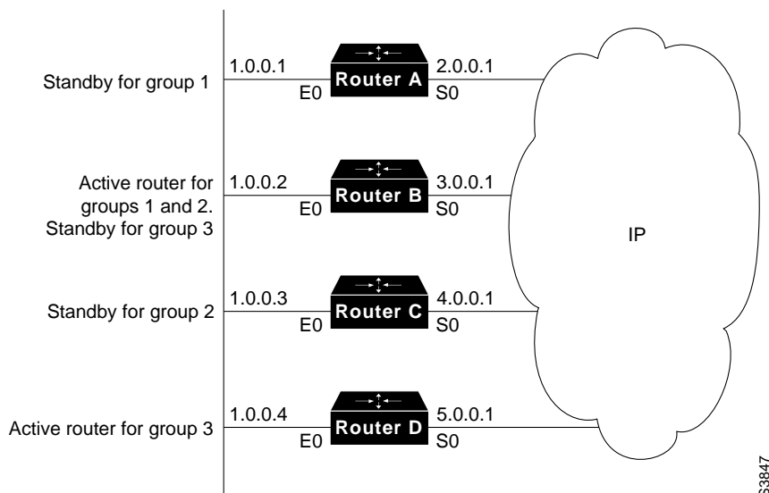
Figure 9-4 Example of Hot Standby Groups
