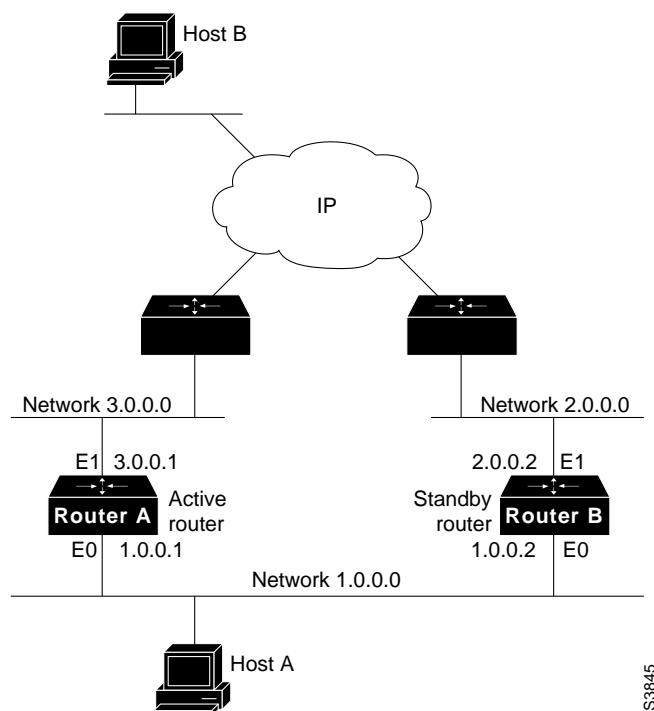
Figure 9-3 Example of a Network Configured for HSRP
